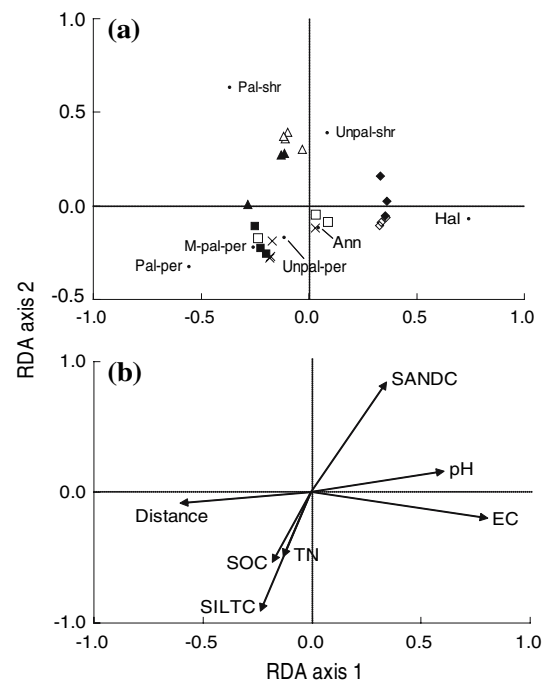
Fig. 5 RDA biplots for (a) functional composition of common survey sites and (b) environmental vectors. MH ( \blacktriangle ), MT ( \blacksquare ), MP ( \square ), MD ( \diamond ), BUP ( \times ), BLP ( \triangle ), and BD ( \blacklozenge ). Plant functional types are marked ( \bullet ). Plant functional types: Pal-shr, palatable shrubs; Unpal-shr, unpalatable shrubs; Pal-per, palatable perennials; M-pal-per, moderately palatable perennials; Unpal-per, unpalatable perennials; Ann, annuals (generally unpalatable); Hal, halophytic shrubs
