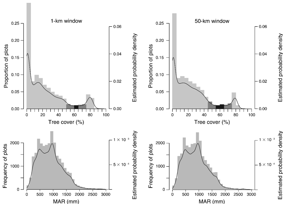
FIG. 1. Histograms of tree cover (%) (top) and mean annual rainfall (MAR; bottom) at 1-km (left) and 50-km scales (right). For histograms of tree cover, dark gray bars denote categories with proportion of plots with values < 2.5\% ; black bars denote the midpoint of the range of dark gray bars. The curves represent the estimated probability density of plots.
