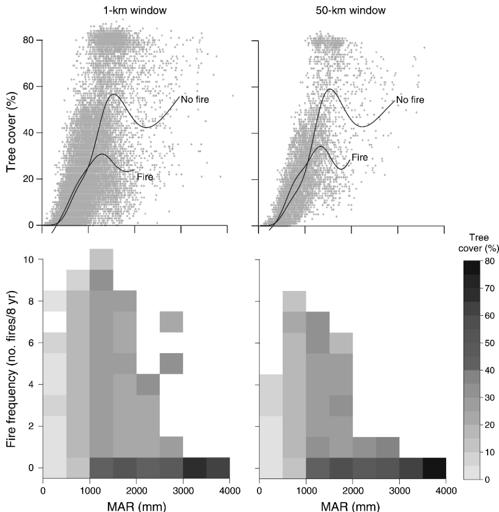
FIG. 4. Effects of rainfall and fire on tree cover in sub-Saharan Africa. (Top panels) tree cover vs. mean annual rainfall at 1-km and 50-km scales. Curves represent fits from generalized additive models including rainfall and fire presence as variables (Table 1); fits are significant at both the 1-km ( R^2 = 0.574 , P < 0.001 ) and the 50-km scale ( R^2 = 0.673 , P < 0.001 ). (Bottom panels) mean percent tree cover vs. rainfall and fire frequency at 1-km and 50-km scales.
