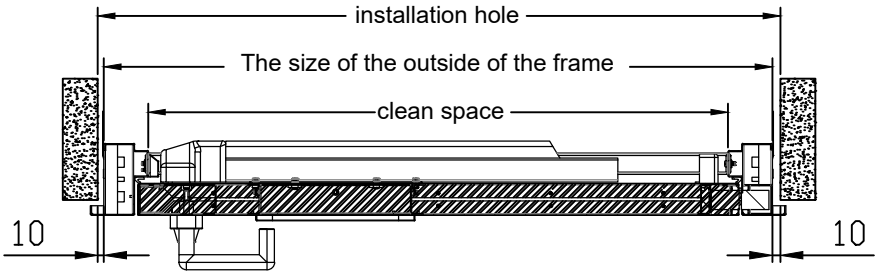
View from the door with a single model
