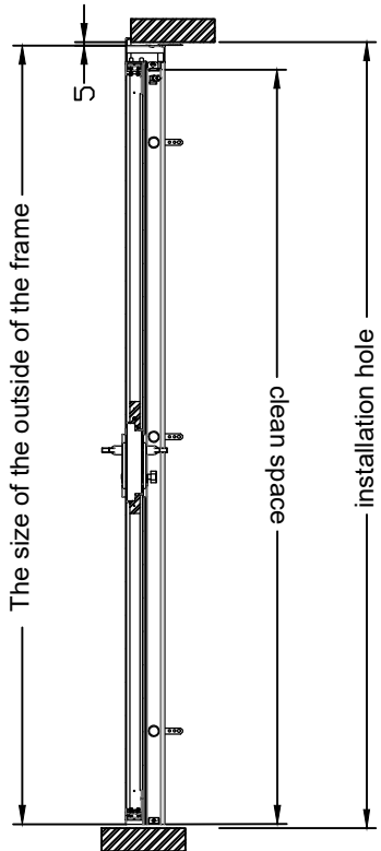
View from the cross section of a single-model door
