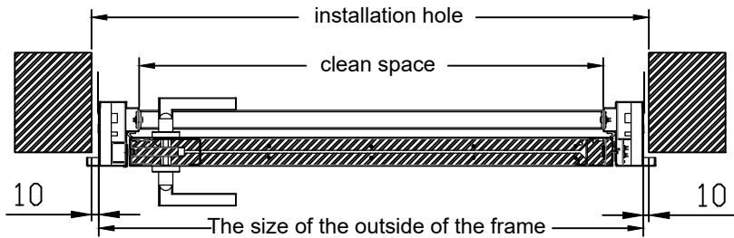
View from the door with a single model
