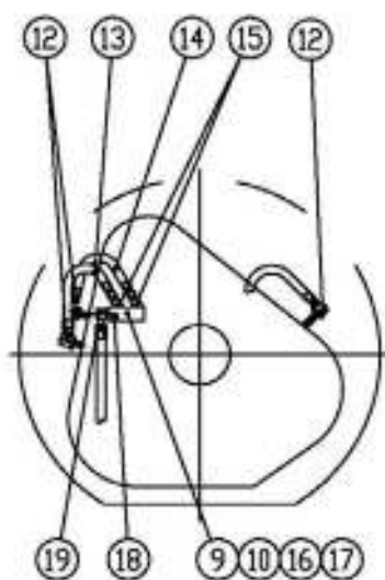
The brake pipe connections of left back wheels
