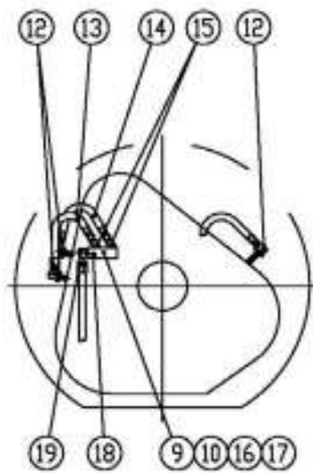
The brake pipe connections of right back wheels
