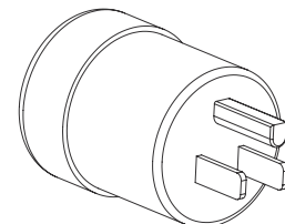
NEMA 5-15 plug (120V only) PLG-515
